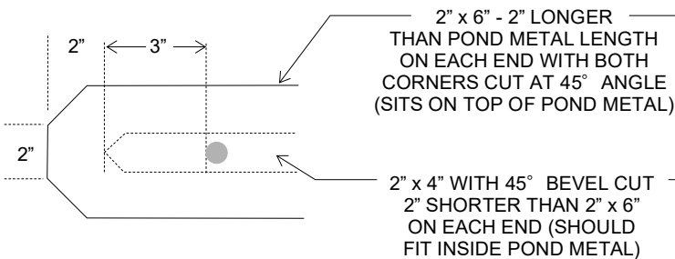
TOP VIEW OF "T" TOP BRACE CROSSBAR
