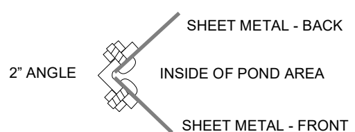
CROSS-SECTION SHOWING POND SHEET METAL ON INSIDE OF 2" ANGLE
